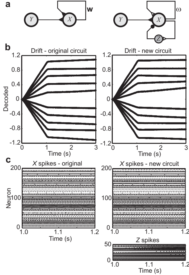
Figure 2: Recurrent networks acting as a neural integrator ( \dot{x} = 0 ). A) Structure of the networks before and after the elimination of negative weights. Neural ensembles are drawn as single units for simplicity. The recurrent synapses \omega are targeted by the transformation. B) Decoded output from a neural integrator before and after the elimination of negative weights. Inputs are 1-second square pulses at various levels and the networks are run for 3 s. The individual curves are from each of 10 distinct simulations. This demonstrates that the network dynamics are largely unaffected by the change in network topologies. C) A section of spike trains for the recurrent neurons and the interneurons, showing characteristic firing patterns.
