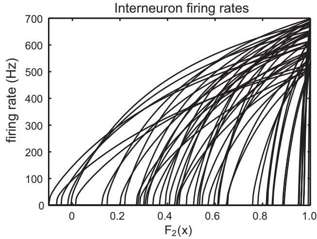
Figure 3: Sample tuning curves for an ensemble of 50 interneurons. The small negative domain allows some neurons to show substantial minimal firing at low values of the positive-only input.
