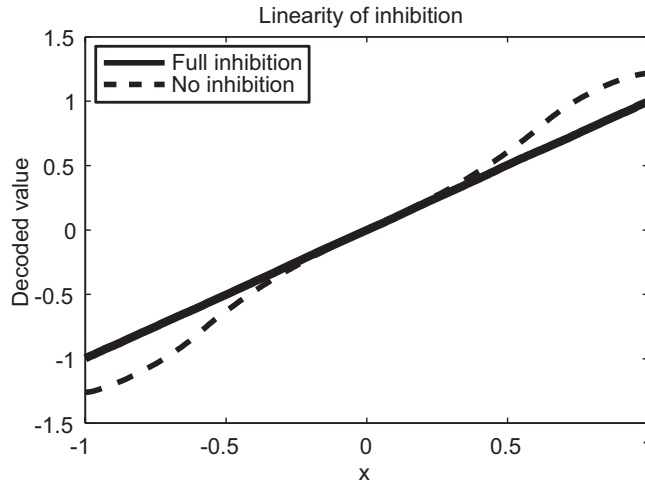
Figure 6: The effects of removing inhibition in a feedforward network. The x-axis is the input to the network and the y-axis is the decoded output for that input. As shown, removing inhibition from the modified network retains good representation at low magnitudes, suggesting that the inhibition primarily linearizes the response at higher magnitudes.
