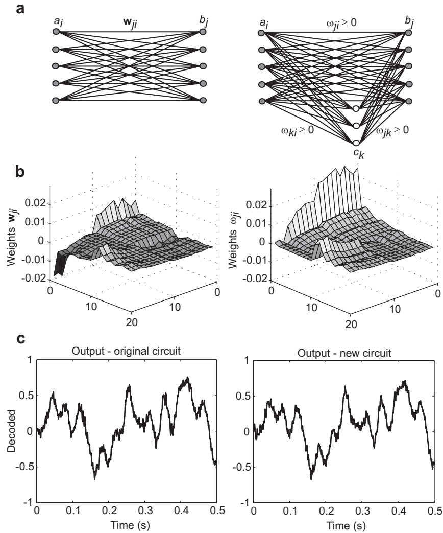
Figure 1: Feedforward networks computing the identity function ( b(x) = x ). A) Structure of the networks before and after the elimination of negative weights. The neurons a_i , b_j , and c_k form the populations A , B , and C , respectively. B) Synaptic weights for an example with 20-neuron excitatory populations. C) Decoded output from the 20-neuron examples, stimulated with 30Hz bandlimited white noise over 0.5 s. This demonstrates that the information passed is largely unaffected by the change in network topologies.
